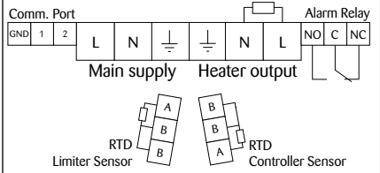
Wiring Details
